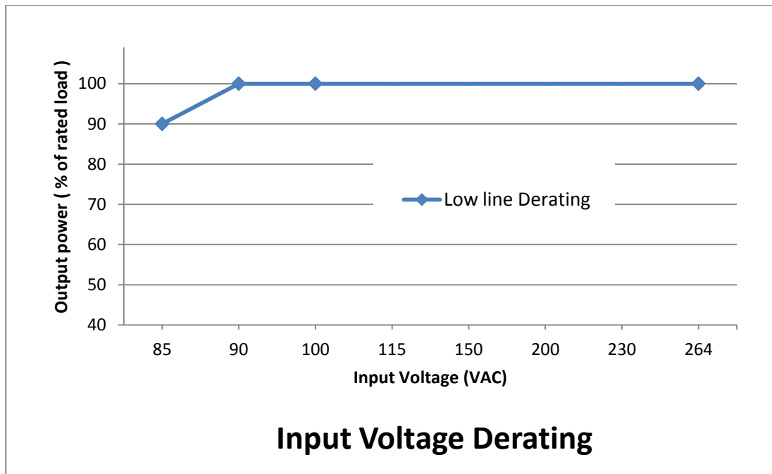
Performance Curves of MPE-T063
